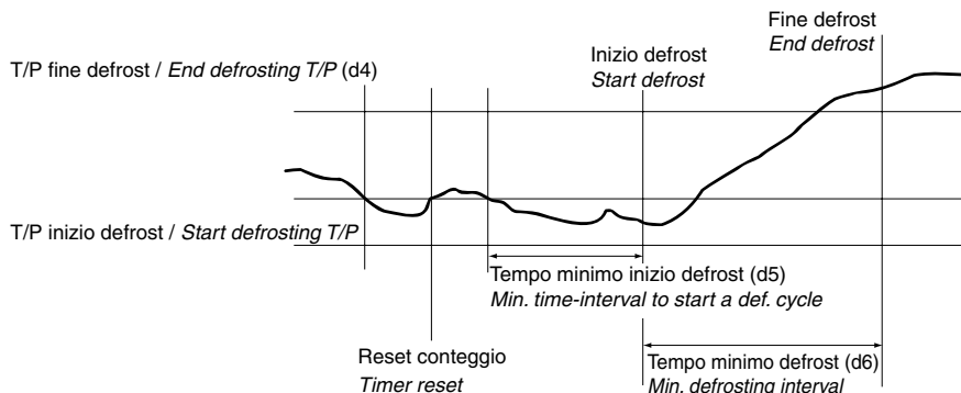
Defrost in temperatura (d2=1) / Temperature-based defrosting (d2=1)
